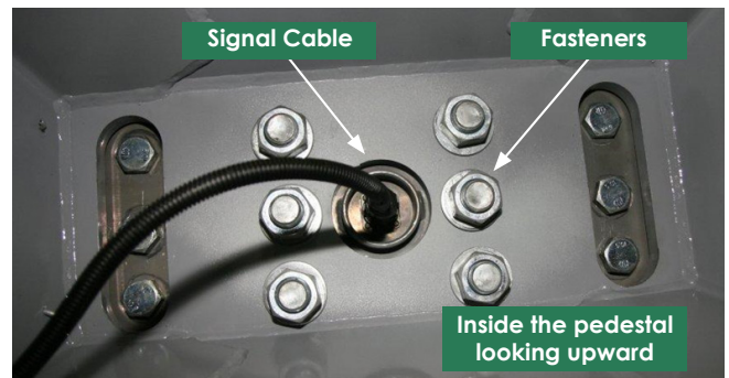
Fasteners connecting mixer scale to the ZF drive
